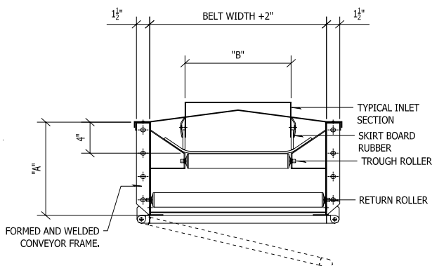
Standard Conveyor Cross-Section.
